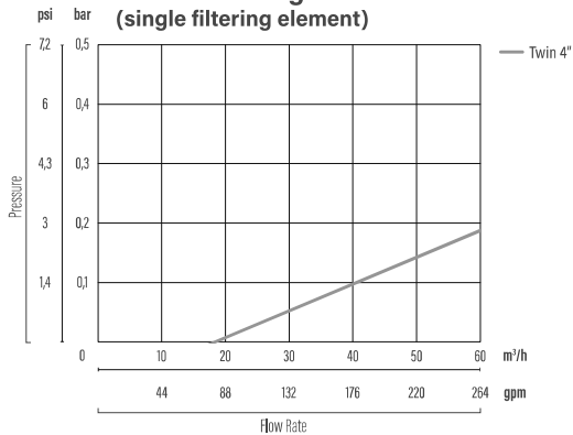
Head loss diagram (single filtering element)
