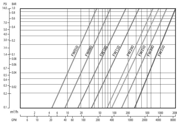
Head loss diagram
