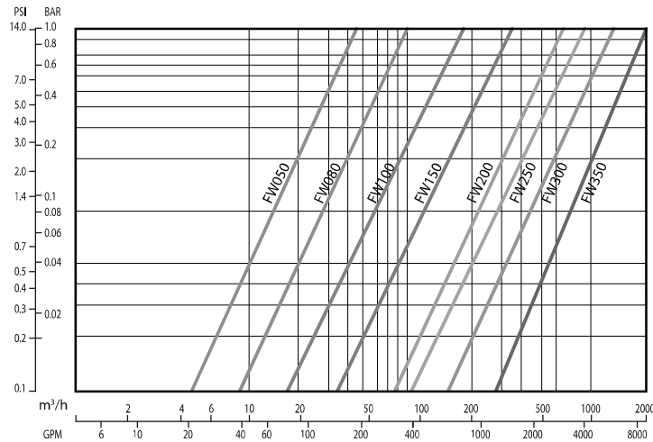
Head loss diagram
