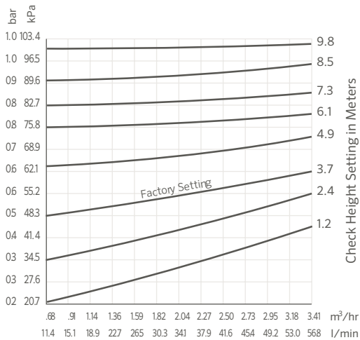
HCV PRESSURE LOSS CHART
